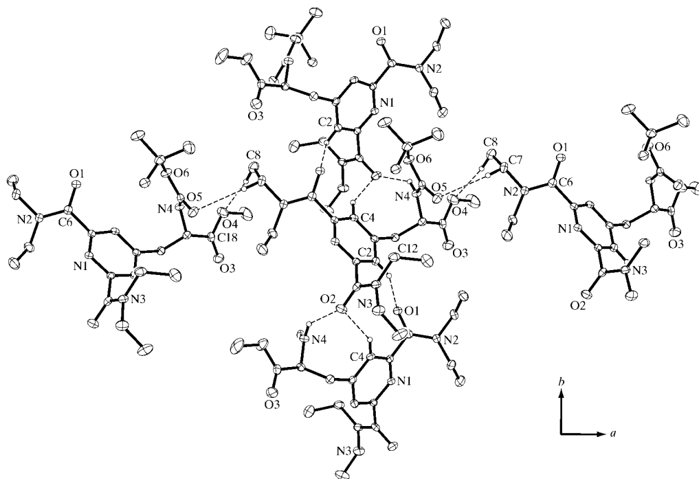
Figure 2 Hydrogen bonds in one of the ab layers. The layer-connecting hydrogen bonds involve O3.
